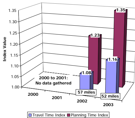
Exhibit SAC-2: 2000 to 2003 Annual Trends
