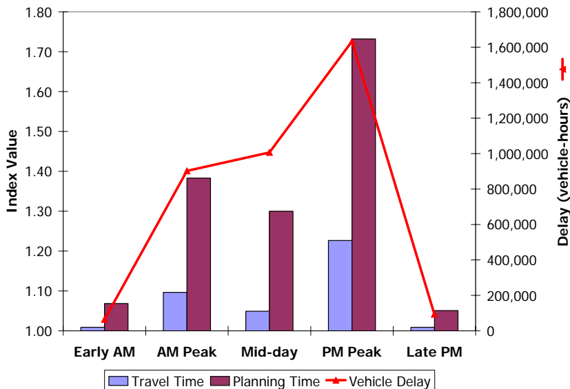
Exhibit SAC-7: Mobility, Reliability, and Delay by Time Period
