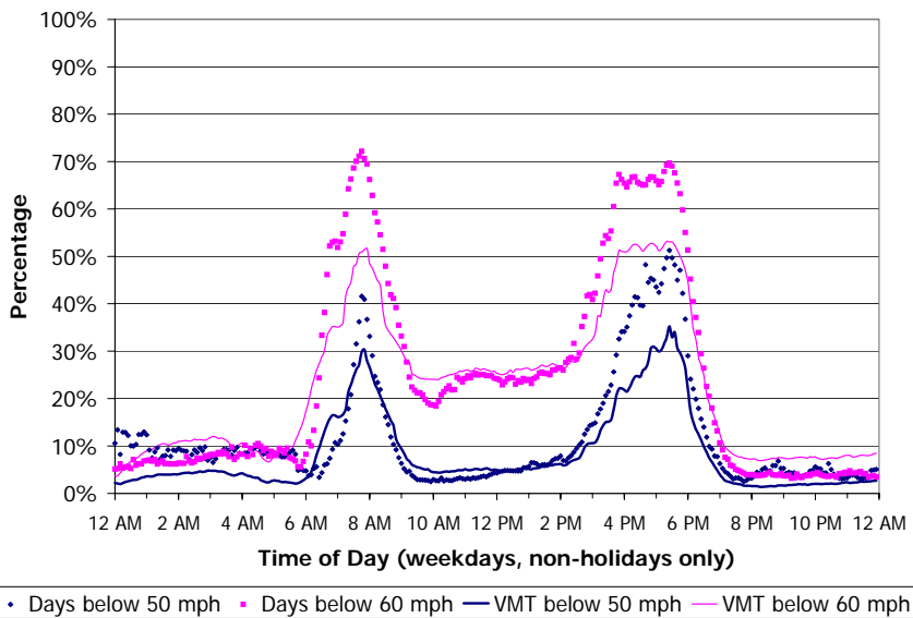
Exhibit SAC-5: Frequency and Percentage of Congested Travel by Time of Average Weekday
