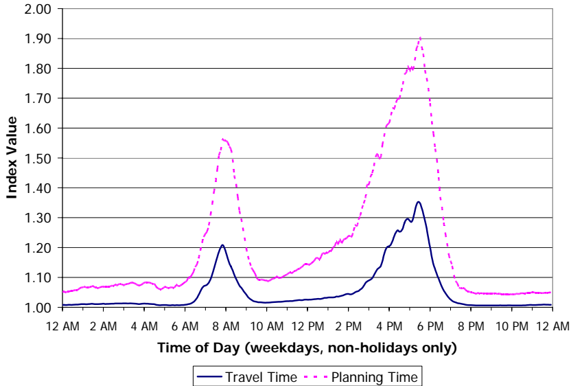
Exhibit SAC-4: Mobility and Reliability by Time of Average Weekday
