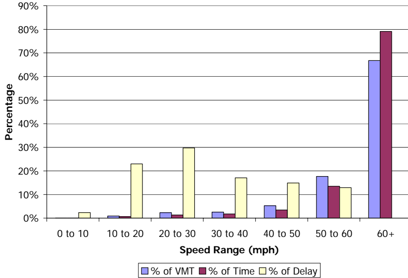
Exhibit SAC-10: Percent of VMT, Delay and Time Periods in Different Speed Ranges
