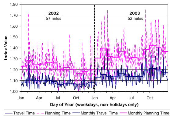
Exhibit SAC-3: Daily and Monthly Trends
